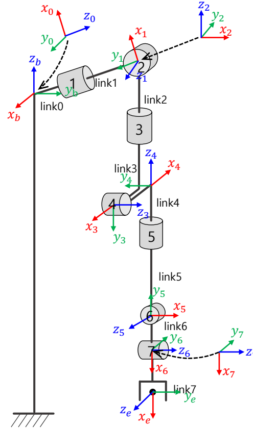
Link & joint numbering Axes and coordinates
