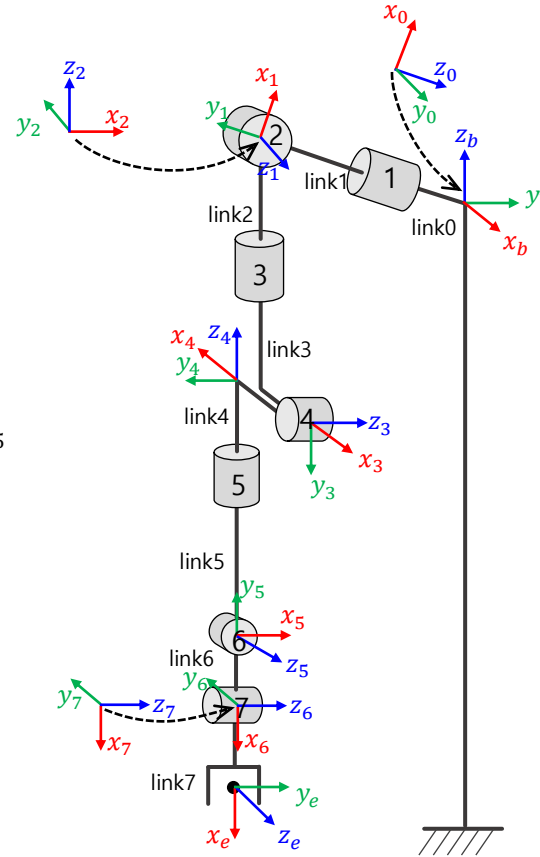
Link & joint numbering Axes and coordinates
